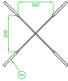
L Foundation bolt/Bulong móng
