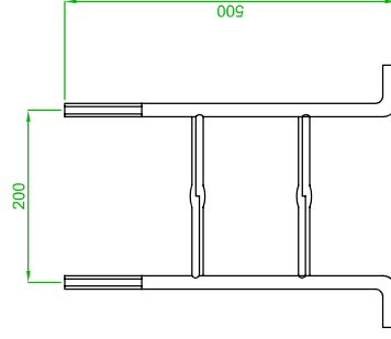
L Foundation bolt / Bulong móng
